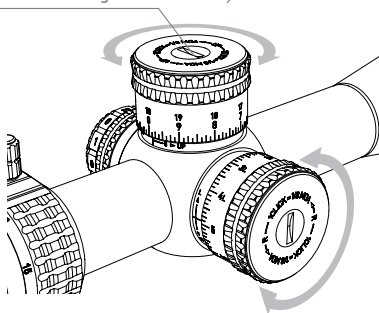
Center Screw of Elevation Turret Knob (Same Design for Windage Turret Knob)
